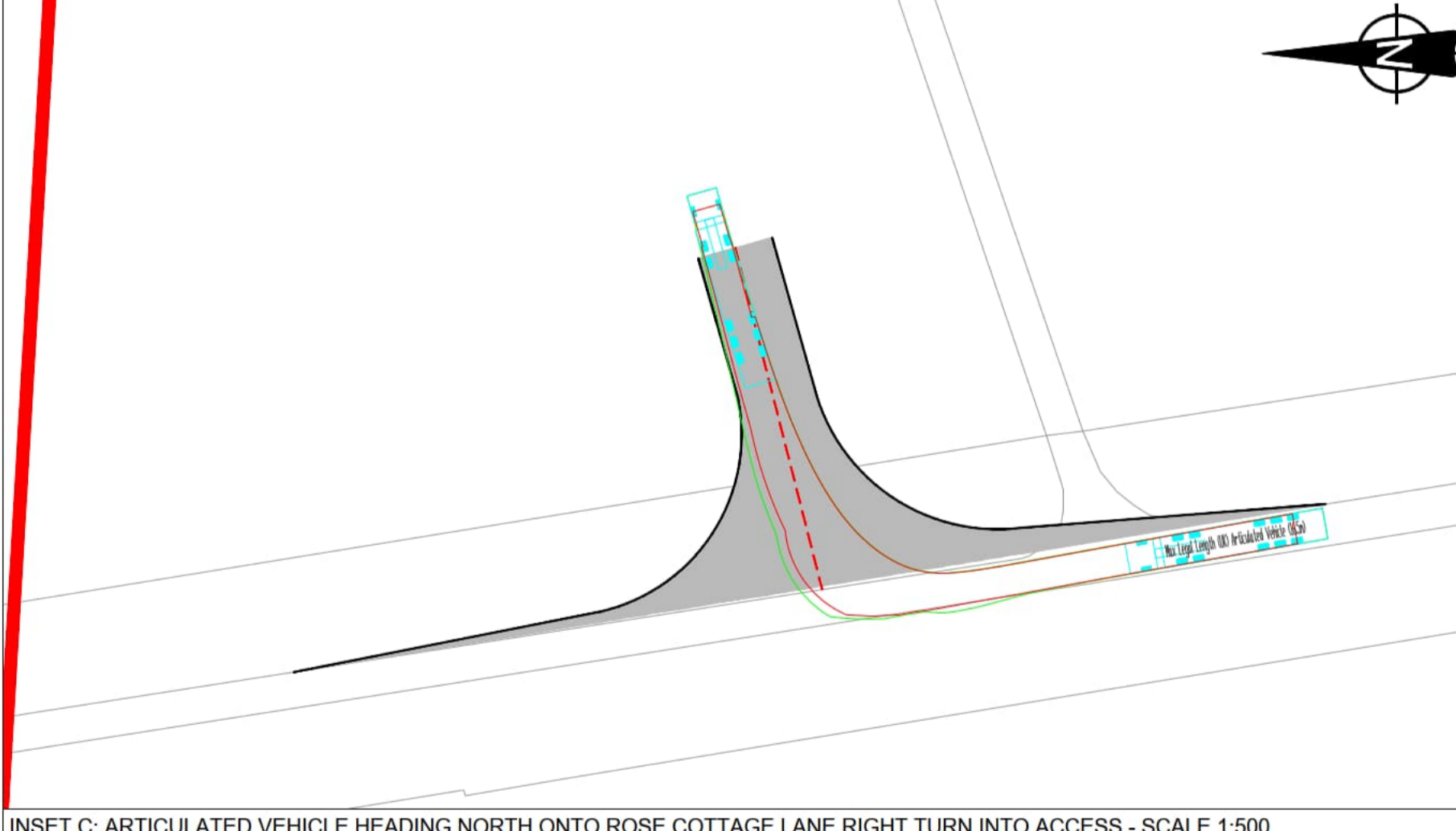
INSET C: ARTICULATED VEHICLE HEADING NORTH ONTO ROSE COTTAGE LANE RIGHT TURN INTO ACCESS - SCALE 1:500
