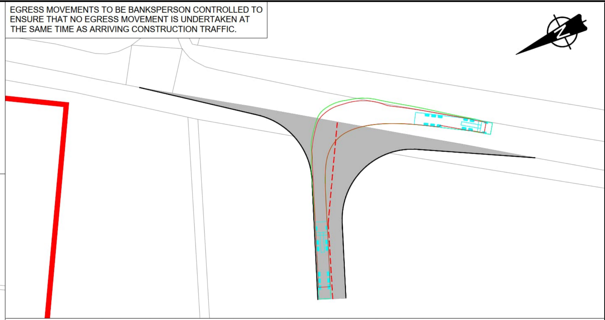
INSET A: ARTICULATED VEHICLE MANOEUVRE RIGHT TURN OUT OF ACCESS ONTO BROUGHTON LANE HEADING SOUTH - SCALE 1:500
