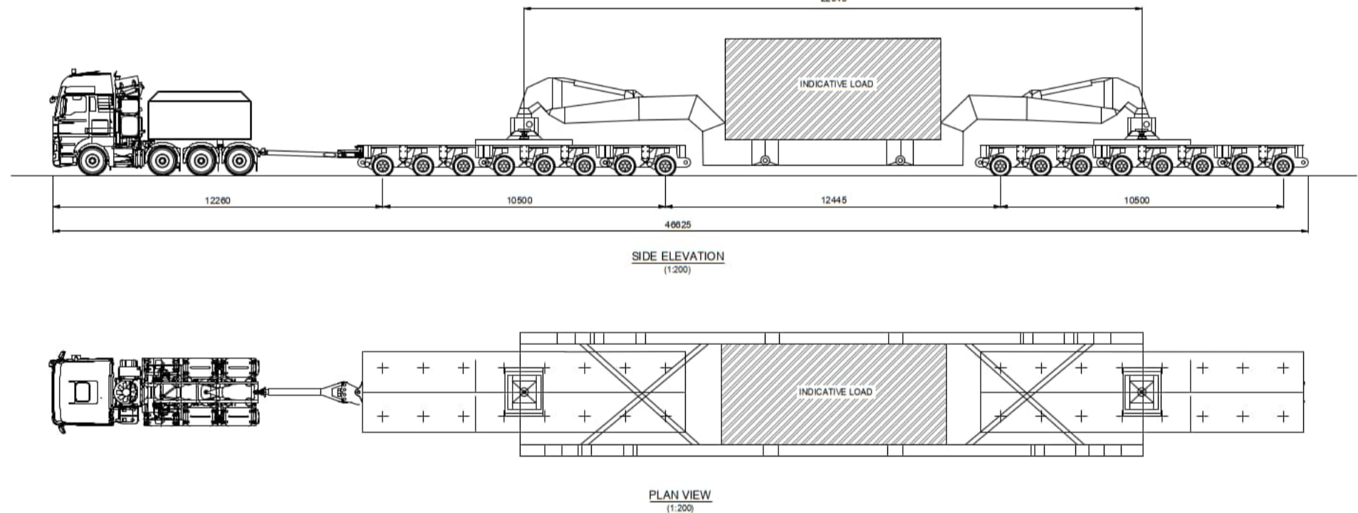
VEHICLE CONFIGURATION - 16-AXLE GIRDER TRAILER (Refer notes)
