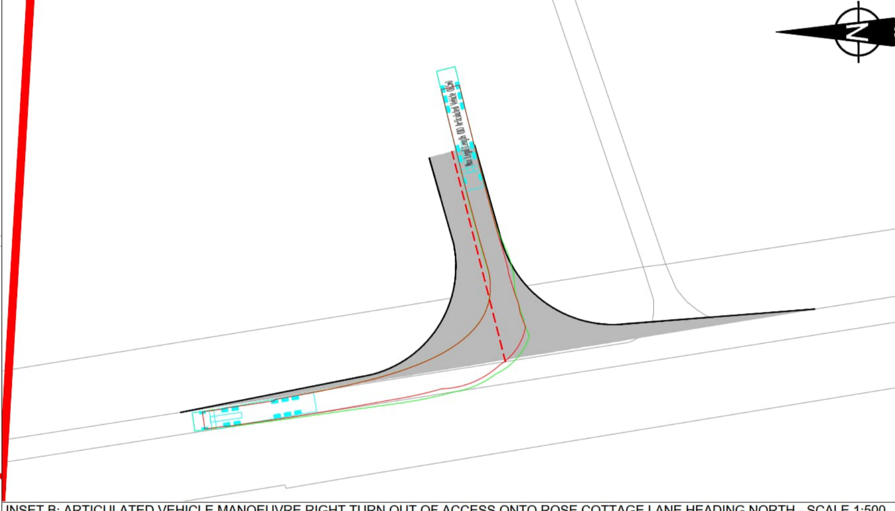
INSET B: ARTICULATED VEHICLE MANOEUVRE RIGHT TURN OUT OF ACCESS ONTO ROSE COTTAGE LANE HEADING NORTH - SCALE 1:500
