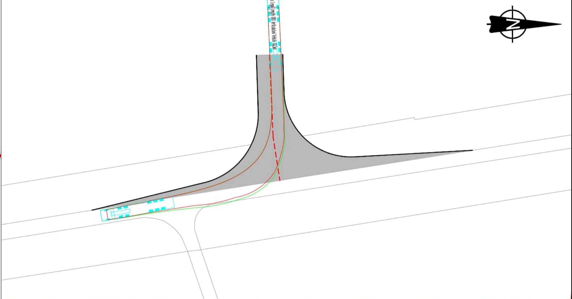
INSET B: ARTICULATED VEHICLE MANOEUVRE RIGHT TURN OUT OF ACCESS ONTO ROSE COTTAGE LANE HEADING SOUTH - SCALE 1:500
