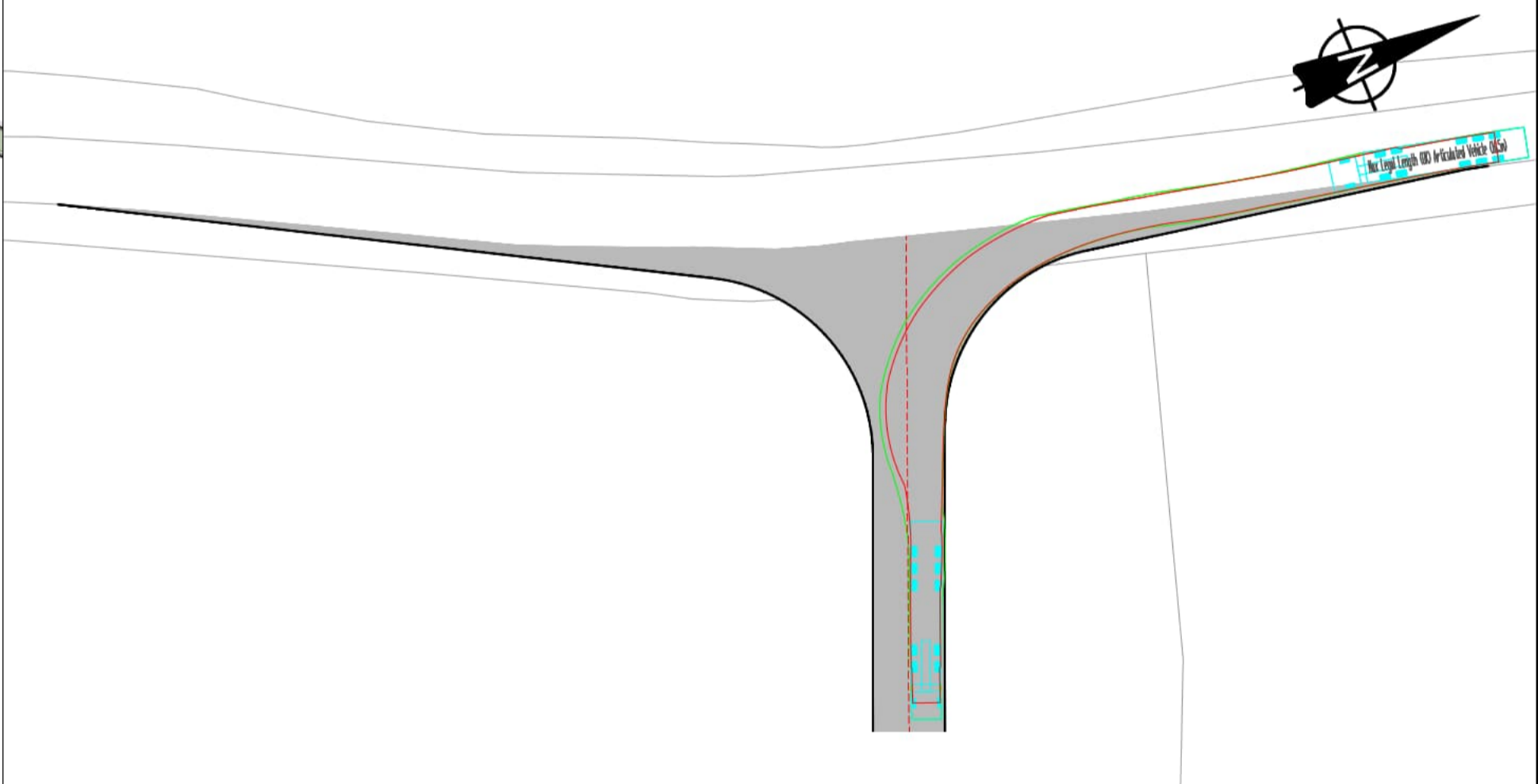
INSET C: ARTICULATED VEHICLE HEADING SOUTH ON HADDINGTON LANE LEFT TURN INTO ACCESS - SCALE 1:500
