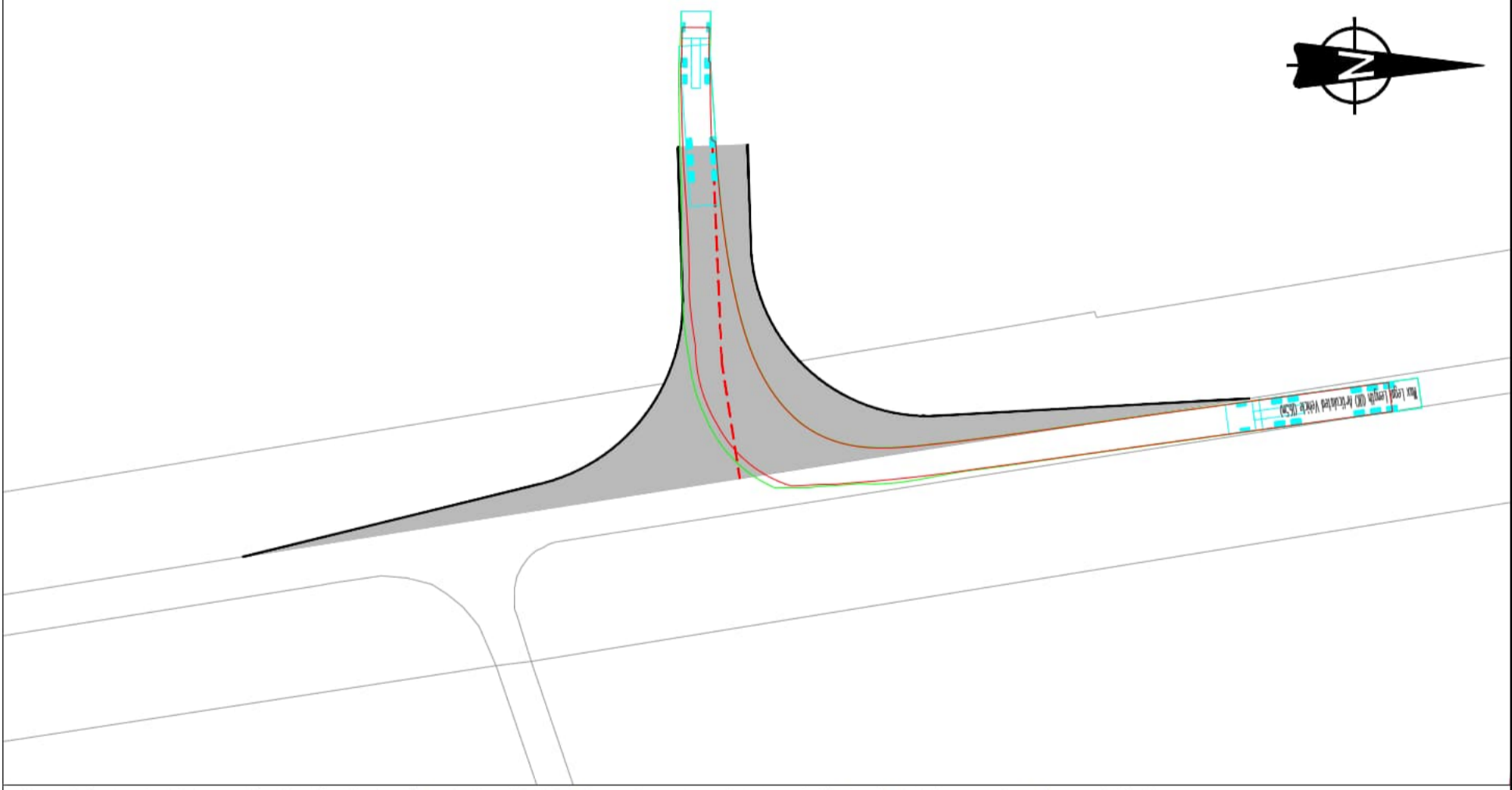
INSET C: ARTICULATED VEHICLE HEADING SOUTH ON ROSE COTTAGE LANE RIGHT TURN INTO ACCESS - SCALE 1:500
