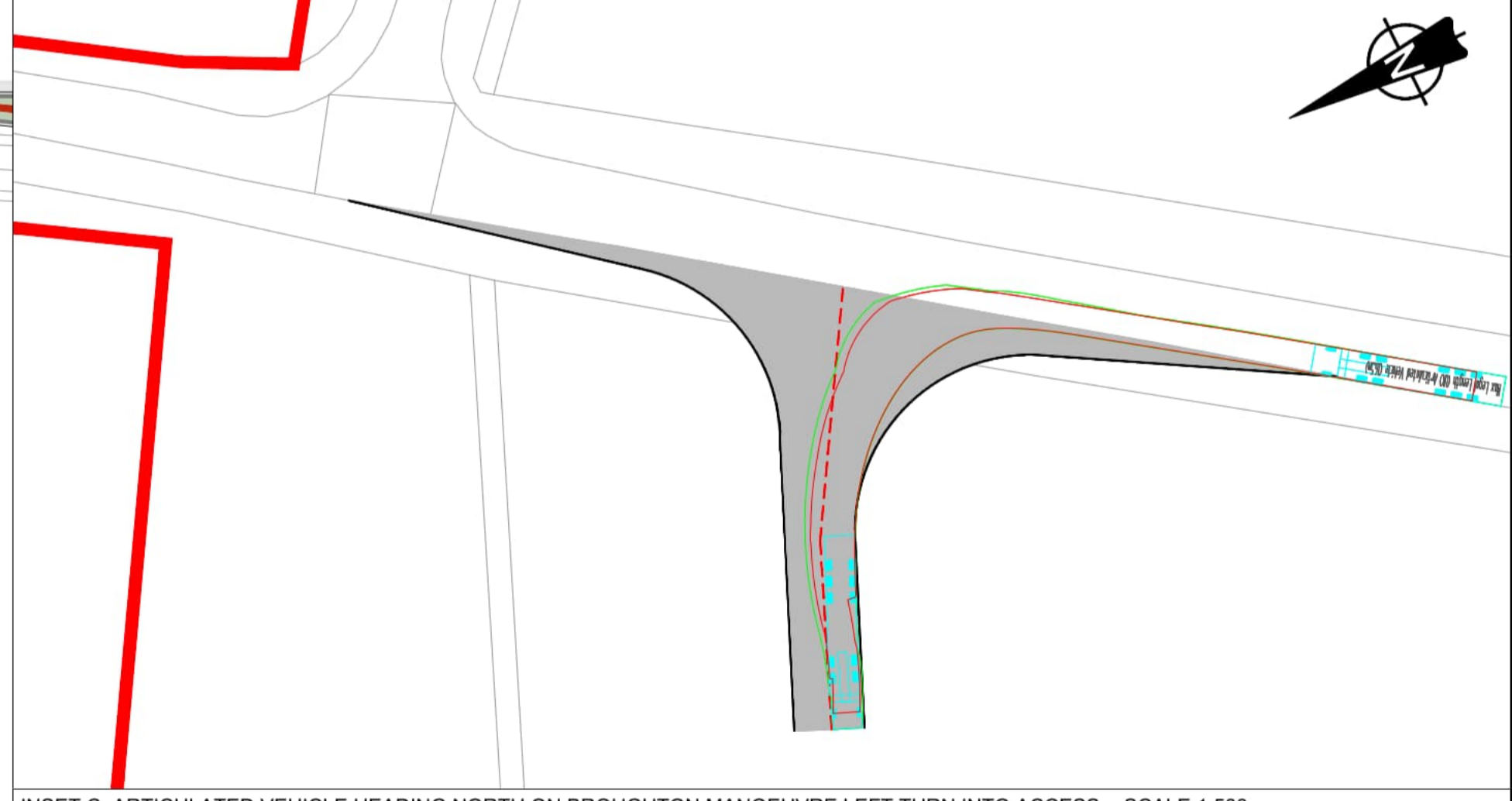
INSET C: ARTICULATED VEHICLE HEADING NORTH ON BROUGHTON MANOEUVRE LEFT TURN INTO ACCESS - SCALE 1:500
