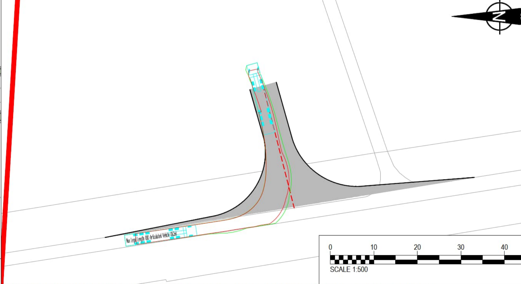
INSET D: ARTICULATED VEHICLE HEADING SOUTH ON ROSE COTTAGE LANE LEFT TURN INTO ACCESS - SCALE 1:500
