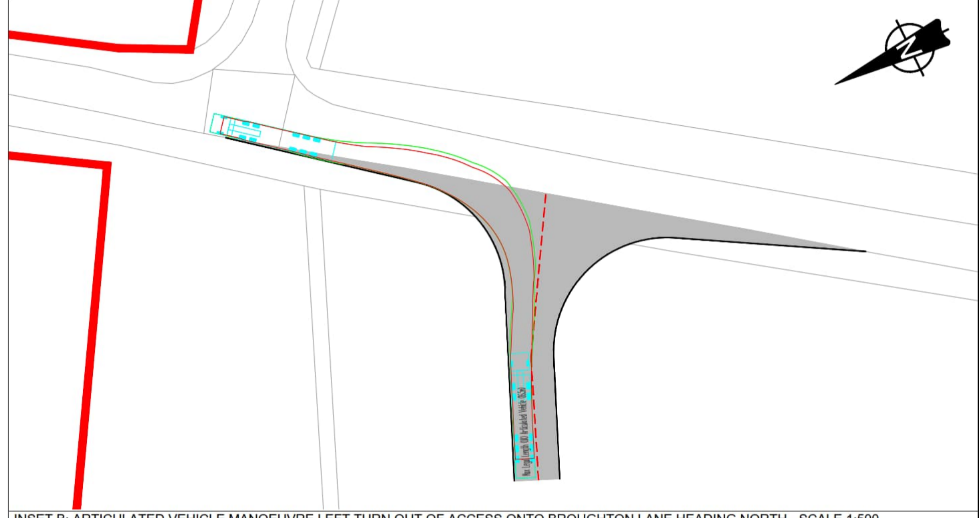
INSET B: ARTICULATED VEHICLE MANOEUVRE LEFT TURN OUT OF ACCESS ONTO BROUGHTON LANE HEADING NORTH - SCALE 1:500
