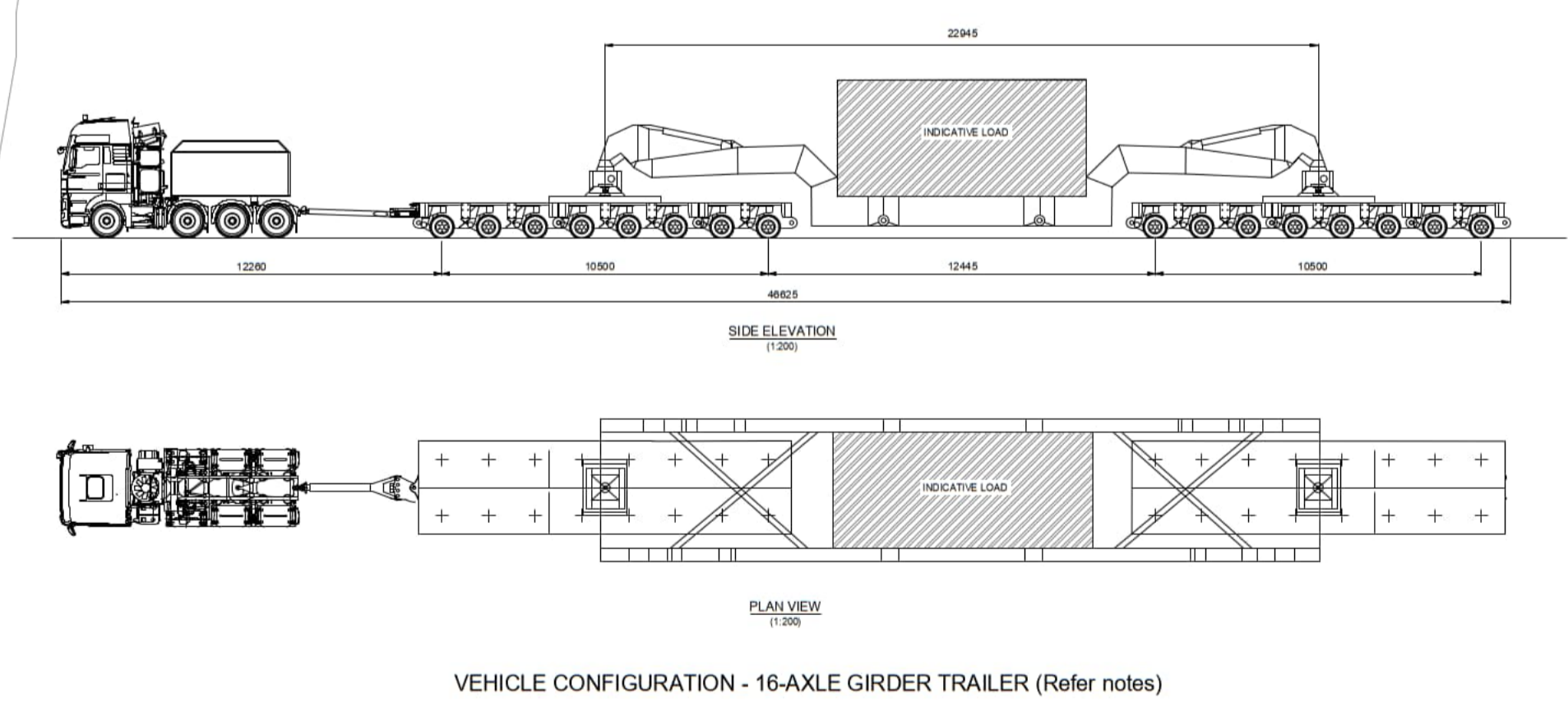
VEHICLE CONFIGURATION - 16-AXLE GIRDER TRAILER (Refer notes)
