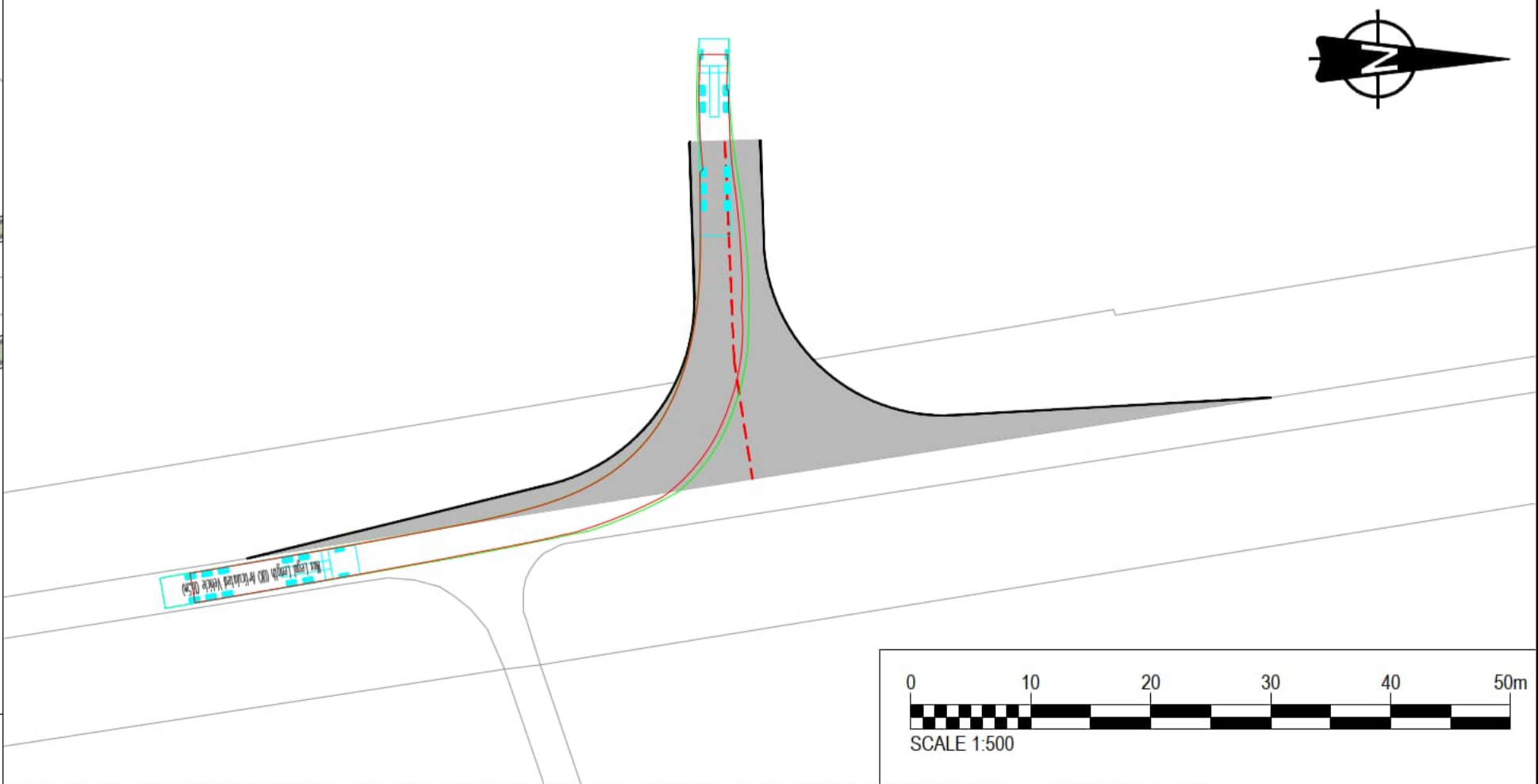
INSET D: ARTICULATED VEHICLE HEADING NORTH ON ROSE COTTAGE LANE LEFT TURN INTO ACCESS - SCALE 1:500
