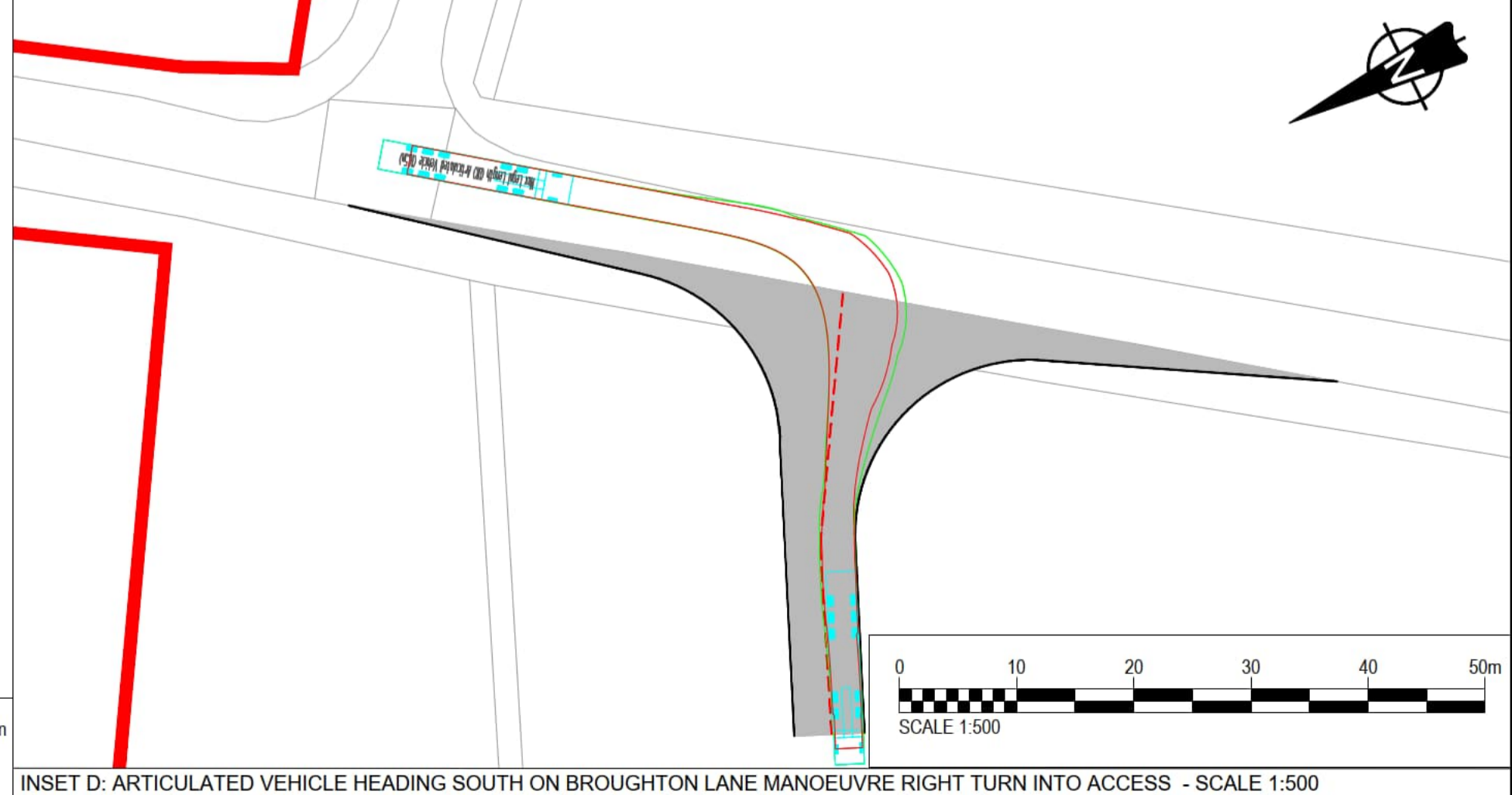
INSET D: ARTICULATED VEHICLE HEADING SOUTH ON BROUGHTON LANE MANOEUVRE RIGHT TURN INTO ACCESS - SCALE 1:500
